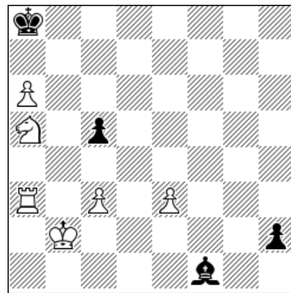
= 1. ♘c4(1) ♗xc4 2. ♖a1 ♗d5 3.e4(1) ♗xe4 4. ♗b3 ♖a7 5. ♗c4(1) ♖b6 6.a7 h1 ♖ 7.a8 ♖ ♗xa8 8. ♖b1+(2) ♖xb1
