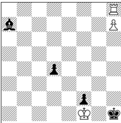
#3 1. ♖b8 ♖h2 2. ♖g8(2) 1... ♗xb8 2.h8 ♖+(3)
